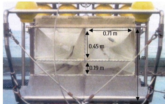
Figure 2: The net used for sampling, indicating net opening dimensions and total height of active sampling area.
