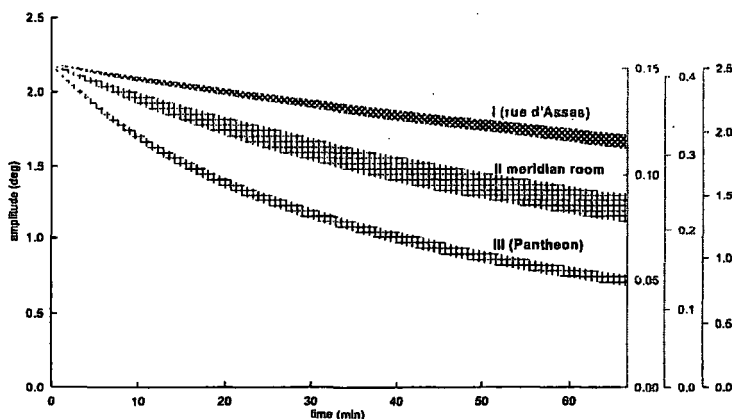
Figure 5. Calculated damping for Foucault's 1851 pendulums. The widths of the traces indicate the ranges expected due to different factors. Based on Fig. 9.26 in Tobin (2003).
