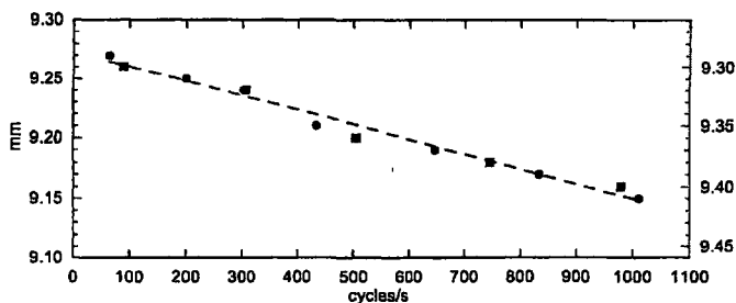
Figure 2. Results of the Foucault rotating mirror experiment. The vertical scales are micrometer readings, the horizontal axis gives the rotation frequency of the mirror in cycles per second. Dots indicate prograde rotation, squares (right axis) are readings from retrograde rotation. The resulting slope (dashed line) is 0.000123 mm per revolution per second.
