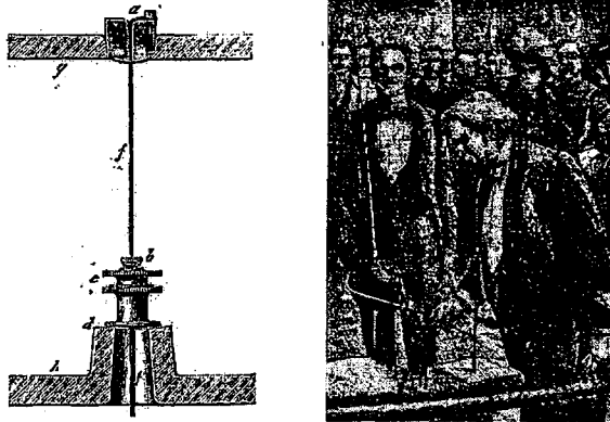
Figure 6. Elimination of disturbances. Left : suspension of the wire of the 1851 Panthéon pendulum ( Receuil des Travaux Scientifiques de Léon Foucault ). Right : Detail of Fig. 4.
